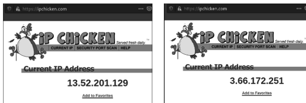
Figure 13-11: IPChicken
